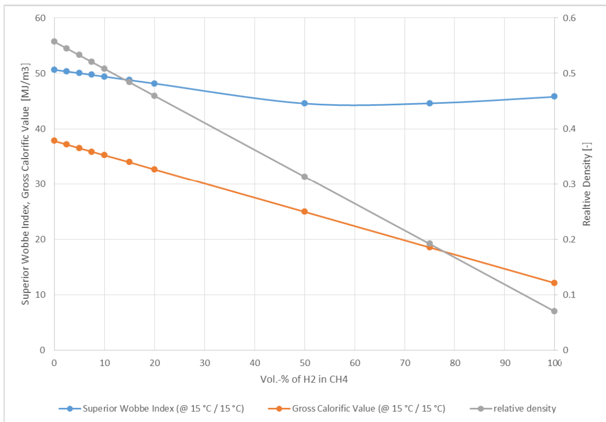
Impact of H 2 concentration in CH 4 /H 2 mixtures on some gas quality properties.
