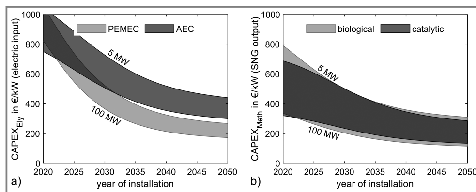
Figure 8. Learning curve and scaling effects for common PtG technologies. a) Electrolysis, b) methanation.
