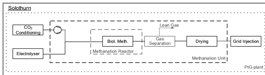
Figure 3. Block flow diagrams of the demo site Solothurn including the chosen system boundaries (dashed lines) for the technical and economic evaluation.
