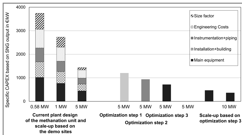
Figure 7. CAPEX_{Meth} calculations for different configurations of the Falkenhagen plant. In a first step, CAPEX_{Meth} was calculated for the demo site. Based on plant design of the demo site, a scale-up to an SNG output of 5 MW was performed. Subsequently, the impact of different optimization potentials on CAPEX_{Meth} was determined. Optimization step 1, reduction of compressor size; optimization step 2, catalyst reduction; optimization step 3, reactor size. Based on the optimized plant design, scale-up was performed.
