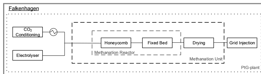
Figure 2. Block flow diagrams of the demo site Falkenhagen including the chosen system boundaries (dashed lines) for the technical and economic evaluation.
