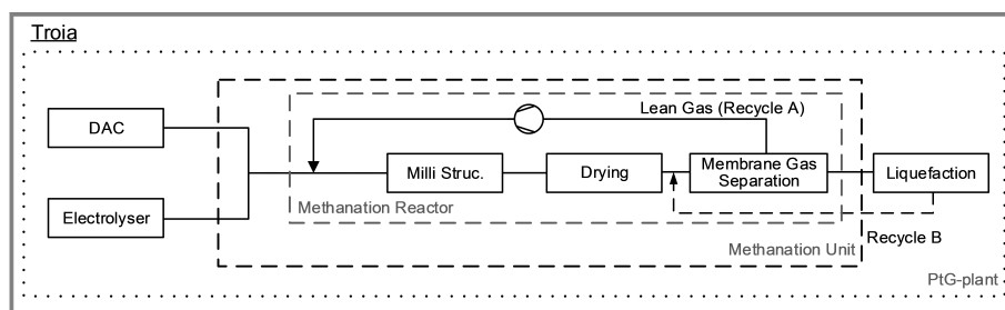
Figure 4. Block flow diagrams of the demo site Troia including the chosen system boundaries (dashed lines) for the technical and economic evaluation.
