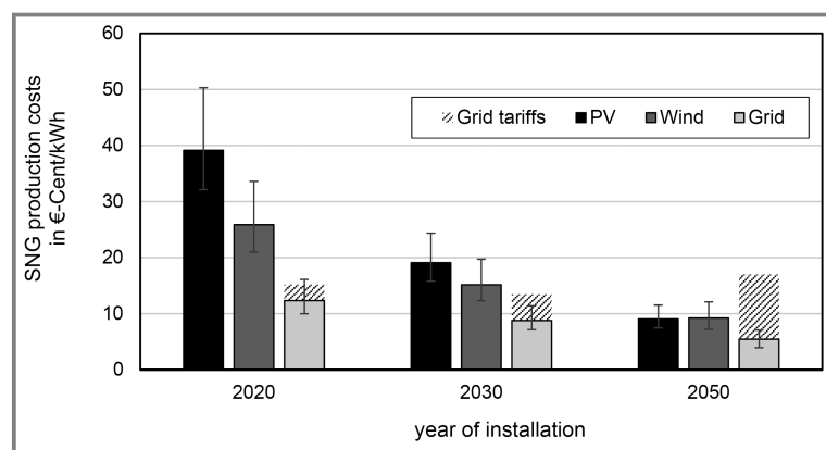
Figure 9. Range of SNG production costs of a 100-MW (nominal electric input) PtG plant in 2020, 2030, and 2050 for different electricity sources.
