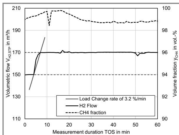
Figure 6. Analysis of the load change rate of the Falkenhagen demo site based on measurement on January 28, 2020. Load change from 71 to 81 %.
