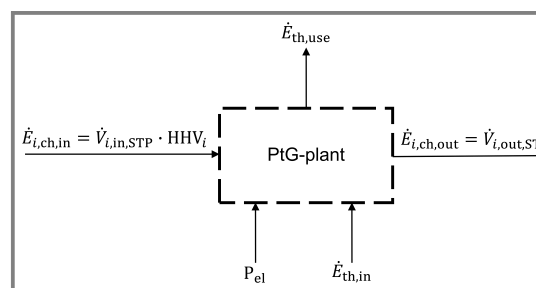
Figure 5. Overview of the general energy flows of a PtG plant.
